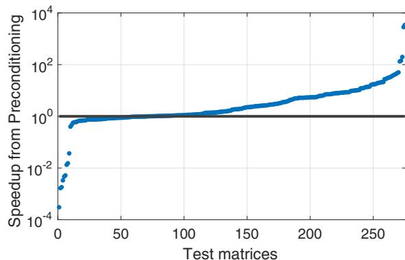
Fig. 3. Speedup obtained from using a Jacobi preconditioner (left side) or an ILU(0) preconditioner over the execution time of the unpreconditioned Krylov solver. Values smaller 1 indicate test cases where the preconditioner increased the solver execution time.
