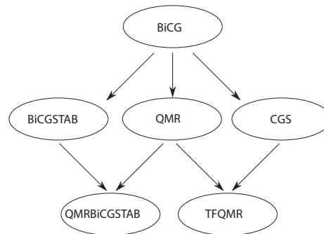
Fig. 1. Outlining dependencies between some Krylov methods based on a Bi-Lanczos process.
