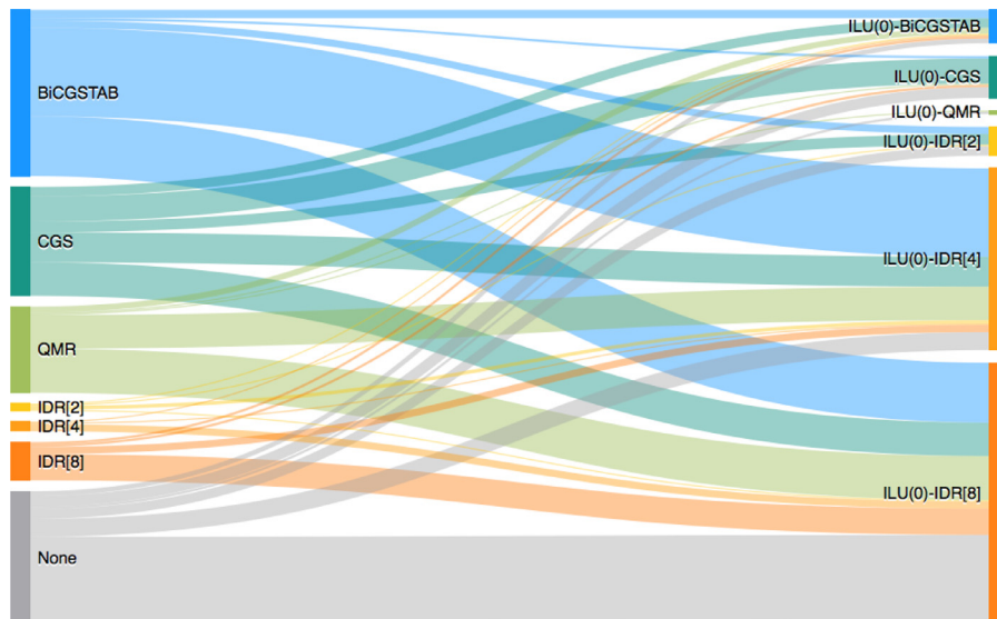
Fig. 8. Choosing the runtime-optimal solver: the height of the bars indicates for how many of the 456 test matrices a certain configuration is the fastest. The solvers on the left do not use any preconditioner; the results on the right use an ILU(0) preconditioner. “None” means that no solver converged within the iteration limit.
